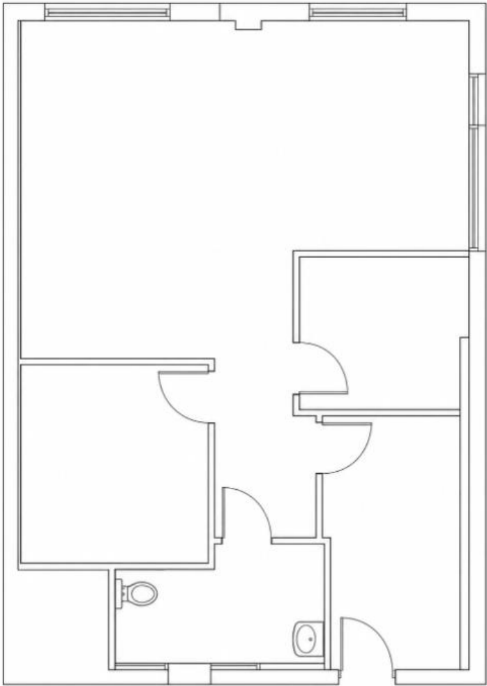
FLOOR PLAN
